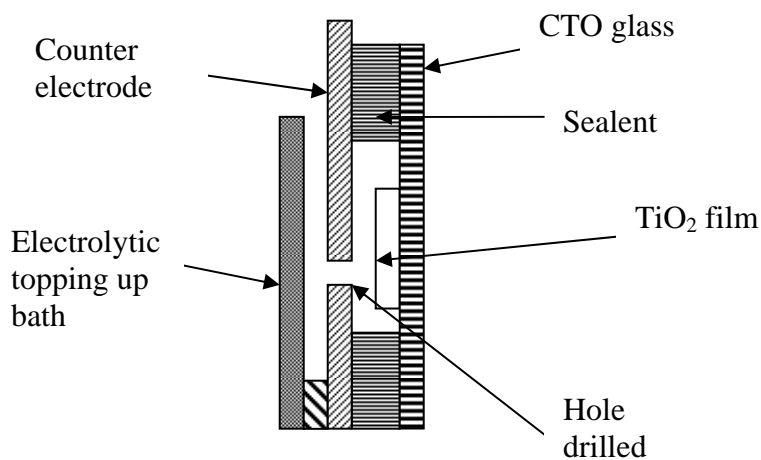
Figure 2: PEC cell with electrolytic topping up bath
