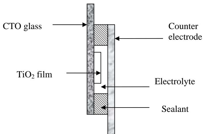
Figure 1 : Typical PEC Cell
